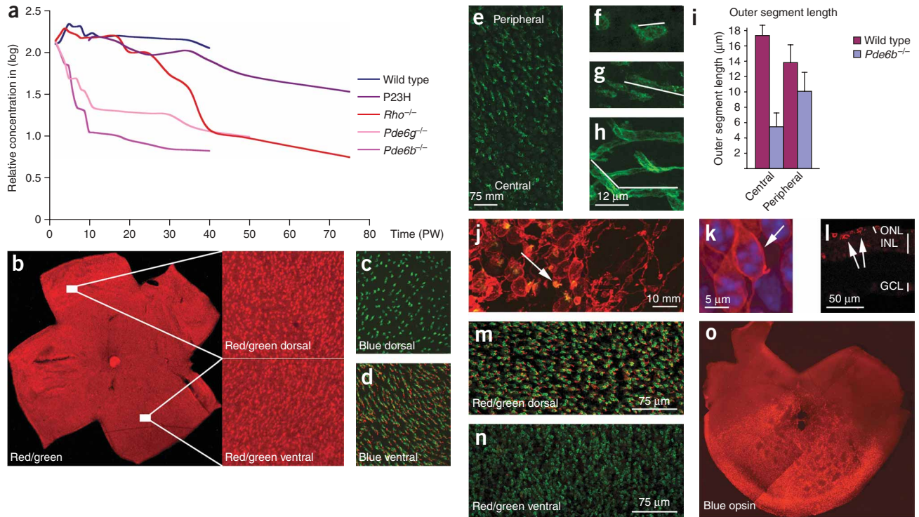
Figure 2 Cone death kinetics. (a) qRT-PCR analysis for Opn1sw during cone degeneration. (b–o) All panels show retinal flat mounts except for i and l. Green signal indicates PNA expression and red signal indicates red/green or blue opsin. The wild-type retina is shown at P35 in b–d. Red/green opsin (b) and PNA (c,d) expression were detected both dorsally and ventrally, whereas blue opsin (c,d) was detected only ventrally. The Pde6b -/- mouse is analyzed in e–g and j–o. A central to peripheral gradient of PNA and shortening of cone outer segments is shown in e–g. At P20, there were fewer elongated outer segments in the center (e) as compared with the periphery. Higher magnifications of a central or peripheral outer segment from e are shown in f and g, and a wild-type outer segment is shown in h (white line marks the outer segment). A quantification of outer segment length at 3 weeks is shown in i (error bars represent s.d. of 15 measurements each). With the shortening of outer segments during degeneration, red/green opsin was localized throughout the membrane of the cell body, and PNA, which detects an extracellular protein(s), was reduced to a small dot attached to the residual outer segment (j) (yellow shows red/green and PNA overlap, arrow). A higher magnification of a cone showing red/green at the membrane is displayed in k (arrow). A cross section showing red/green in cell body is shown in l (arrows) (P70; j–l). During degeneration, red/green opsin was detected mainly dorsally (m), whereas PNA (m, n) or blue opsin (o) expression were not altered (m and n, P21; o, P49). GCL, ganglion cell layer; INL, inner nuclear layer.
